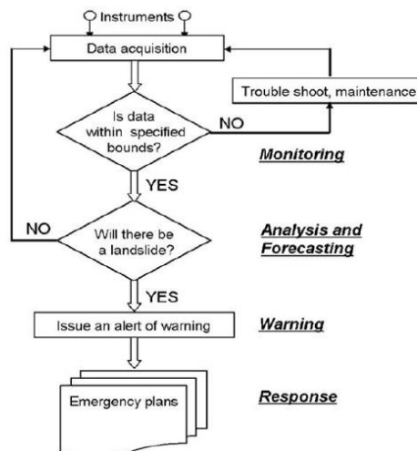
Fig. 2. Block diagram of a typical landslide early warning system DiBiagio & Kjekstad[9]
