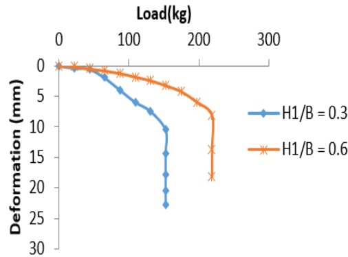
Fig. 4(a). Load deformation curve for Raft
