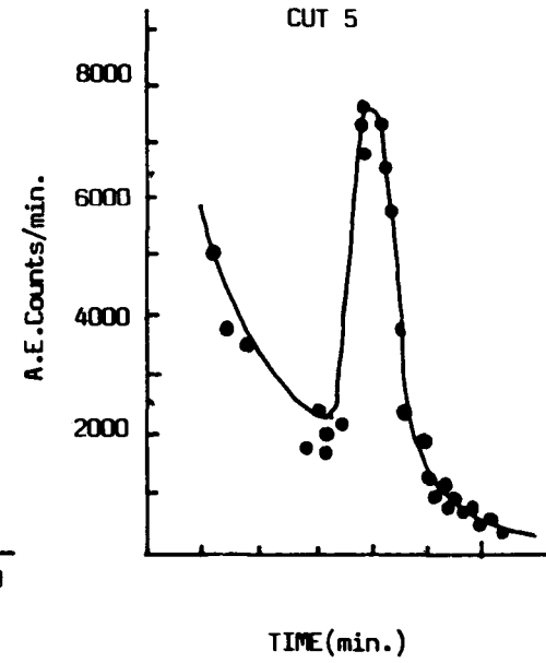
Fig 35: Decay of Ae Count with time as Related to Stability (Koener, McCabe & Lord, 1980)
