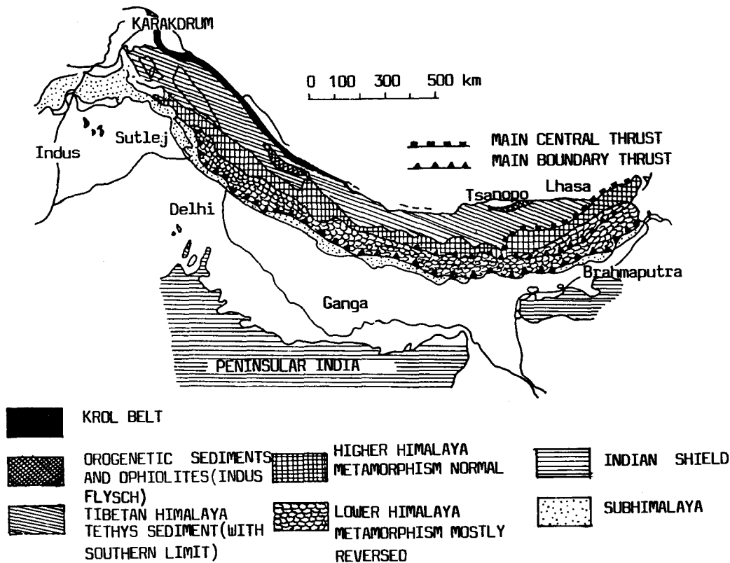
Fig 4: Geological Map of the Himalaya
