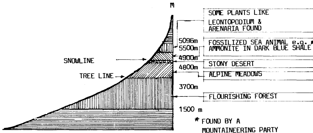
Fig 5: Climatic Variation up the Himalaya
