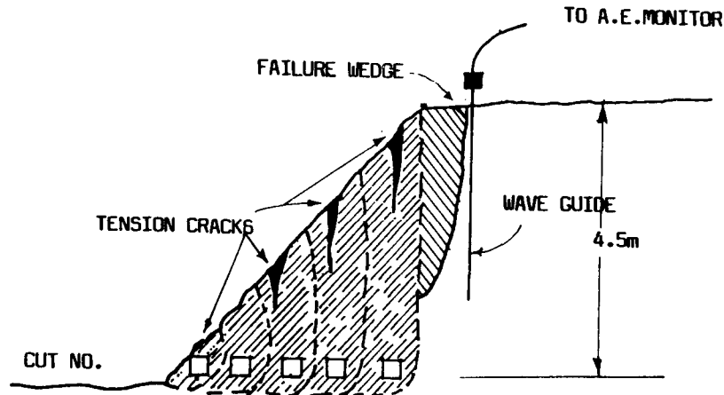
Fig 33: Acoustic Emission Monitoring System
