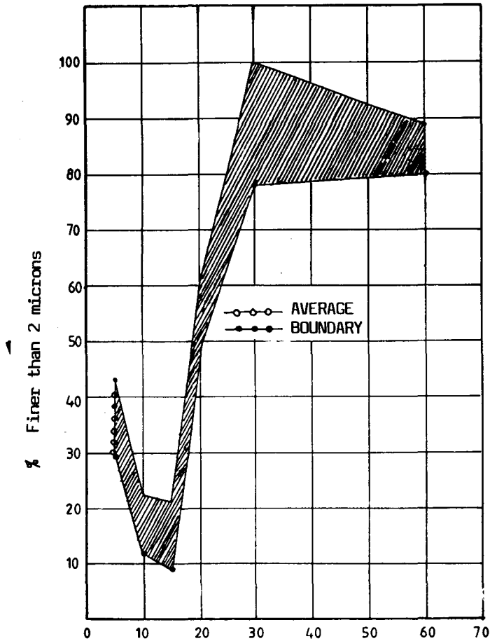
Fig 25: Particle Breakdown due to Large Developments
