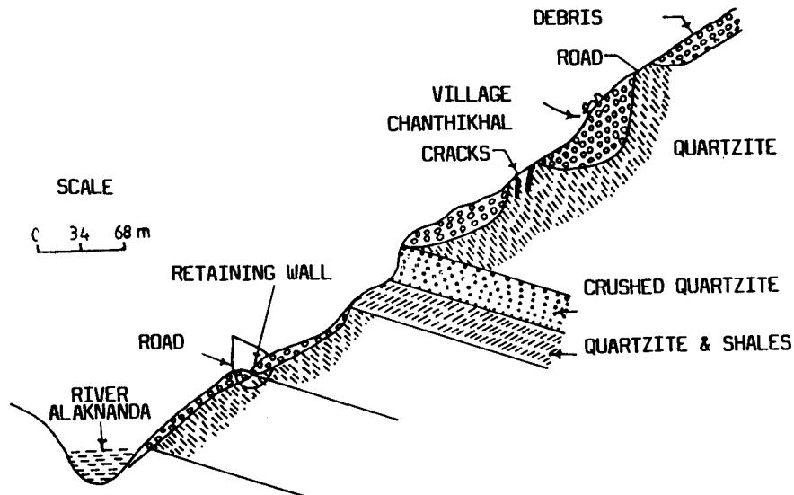
Fig 24: Cross-section of Kaliasaur Landslide at km 187 Hardwar-Badrinath Road
