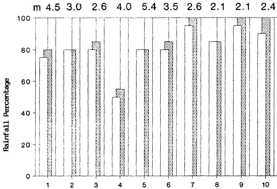
Patterns of Monsoon Rainfall and Winter Precipitation from the Eastern to the western Himalaya
