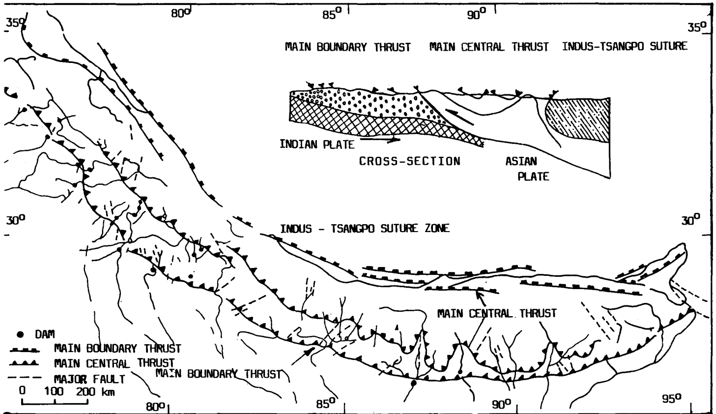
Fig 3: Tectonic Map of the Himalaya (Gansser 1974: Valdiya 1985)
