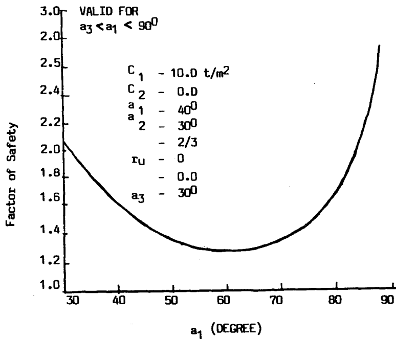
Fig 17: Influence of Orientation of Failure Plane of Factor of Safety
