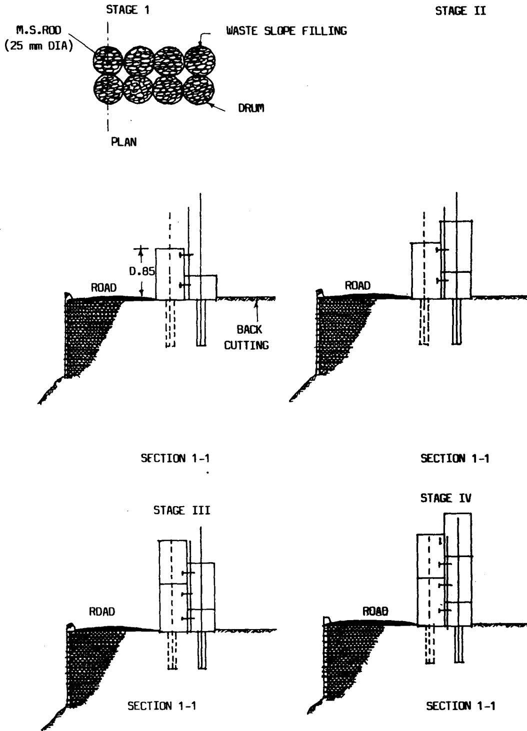
Fig 29: Sequence of Construction of Anchored Drum Diaphragm Wall
