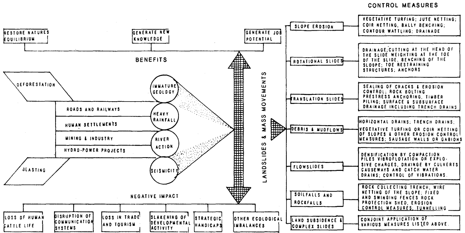
Fig 8: Factors Causing Slope Stability Problems & Common Prescription for their Control
