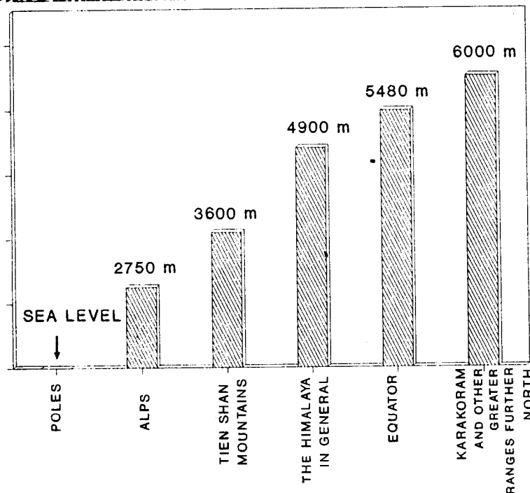
Fig 7: Himalayan Snow Line
