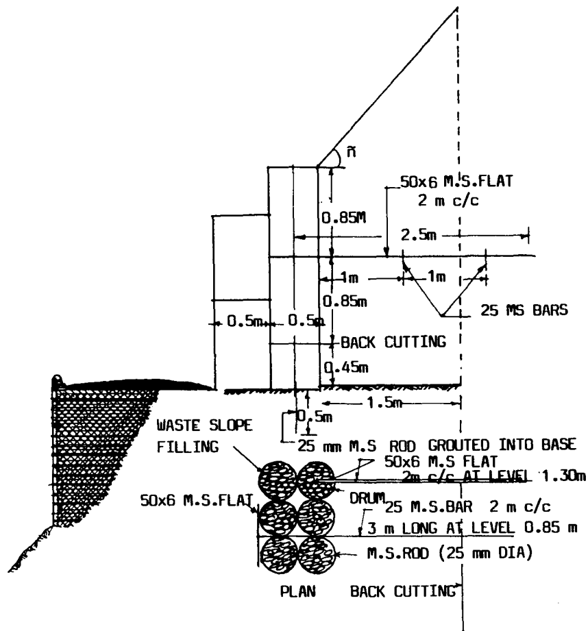
Fig 28: Anchored Drum Diaphragm Wall Built of Slope Waste and Empty Bitumen Drums
