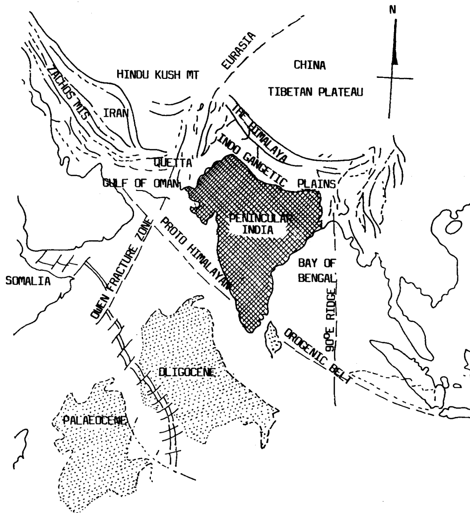
Fig 2: Tectonic Movement of Indian Subcontinent & Birth of the Himalaya (Following Farooq & Siddiqui 1981)
