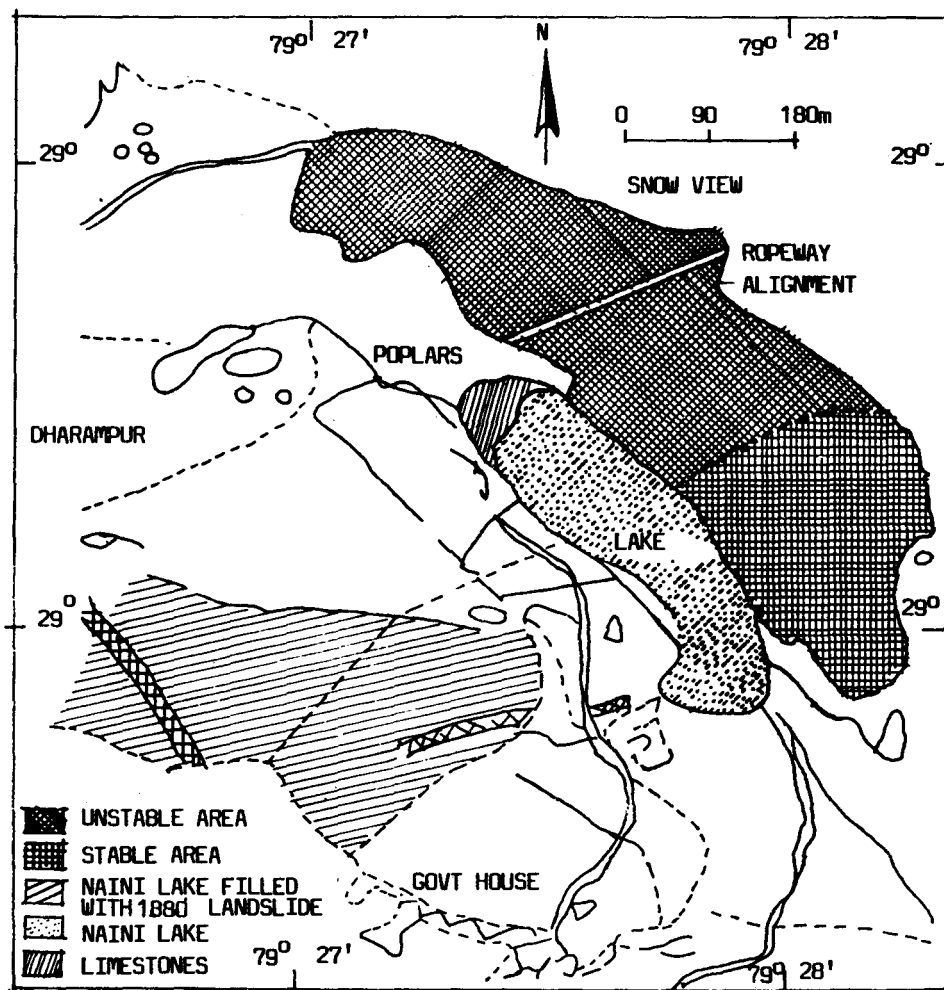
Fig 13: Plan Showing Ropeway Alignment on Sher-Ka-Danda Hill
