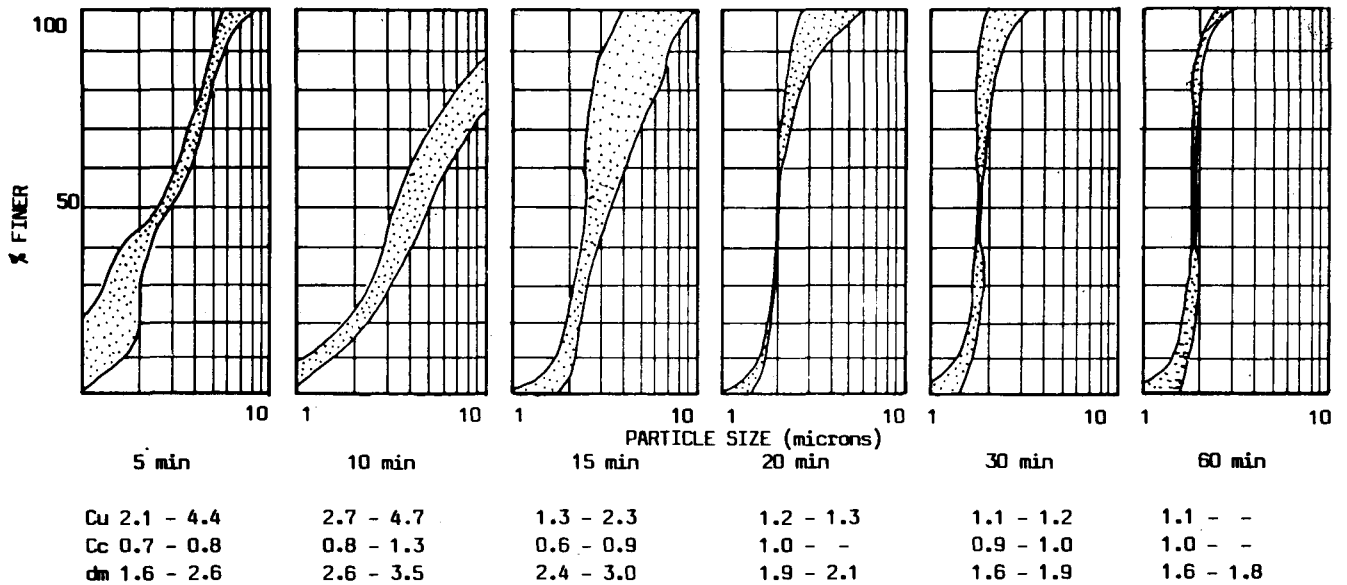
Fig 26: Grain size Variation on Particle Breakdown due to Large Displacements
