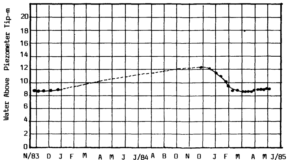
Fig 19:Water Level Above Piezometer Tip T 2 P 3 at 29.5m Below Slope Surface
