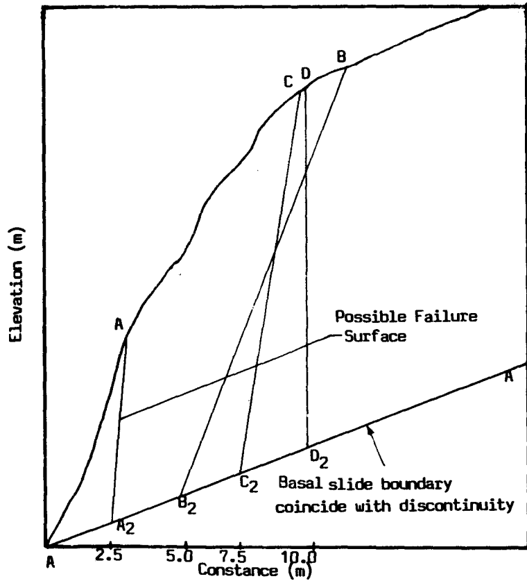
Fig 16: A typical section at T_1 IDEALISED SLOPE PROFILE
