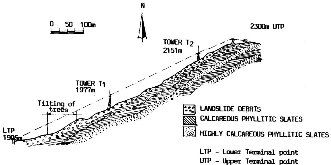
Fig 14: Subslope Profile along the Ropeway Alignment on the Sher-Ka-Danda slope, Nainital (U.P.)
