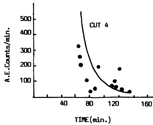
Fig 35: Decay of Ae Count with time as Related to Stability (Koener, McCabe & Lord, 1980)
