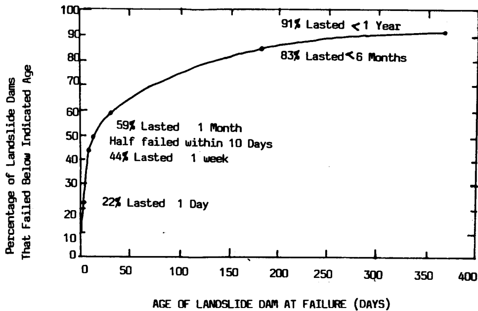
Fig 12: Length of the Landslide Dams Survived 63 Cases from the Literature (Following Schuster, 1986)
