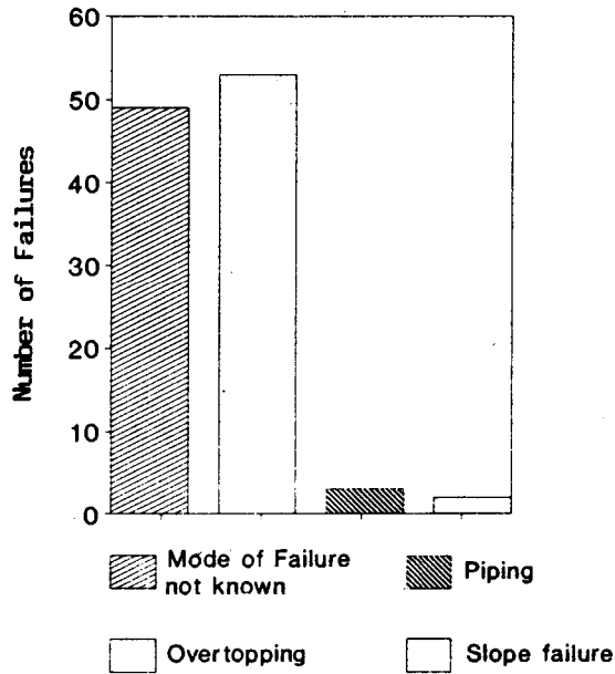
Fig 11: Modes of Failure of Landslide Dams Based on 103 Failures from the Literature (Schuster, 1986)
