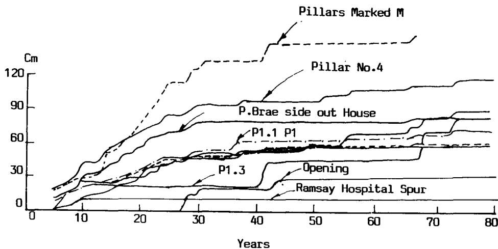
Fig 15: Vertical Movement Record of Markers on the Sher-Ka-Danda hill Nainital
