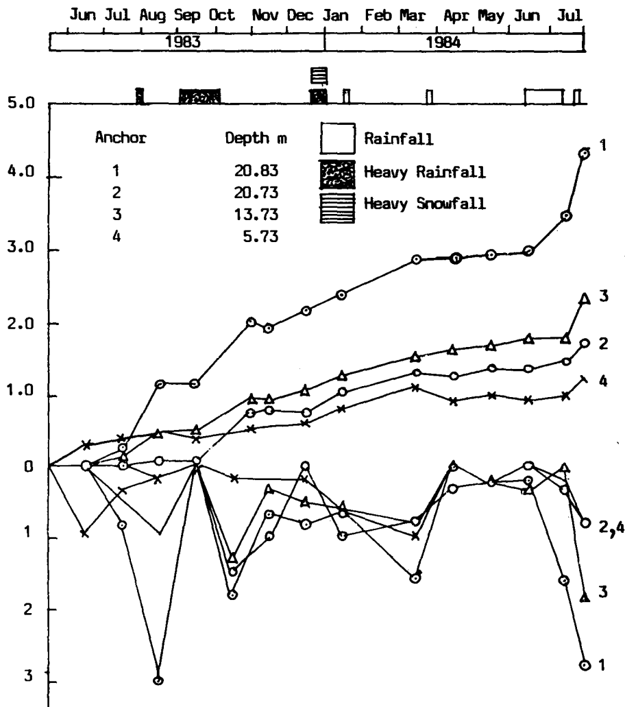
Fig 20: Variation of Total Relative Displacement & Rate of Relative Displacement with Time Near Tower T_1
