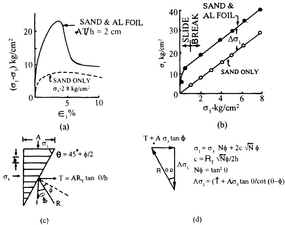
FIGURE 3. Strength of Reinforced Sand Specimens (After Schlosser and Long, 1974)
