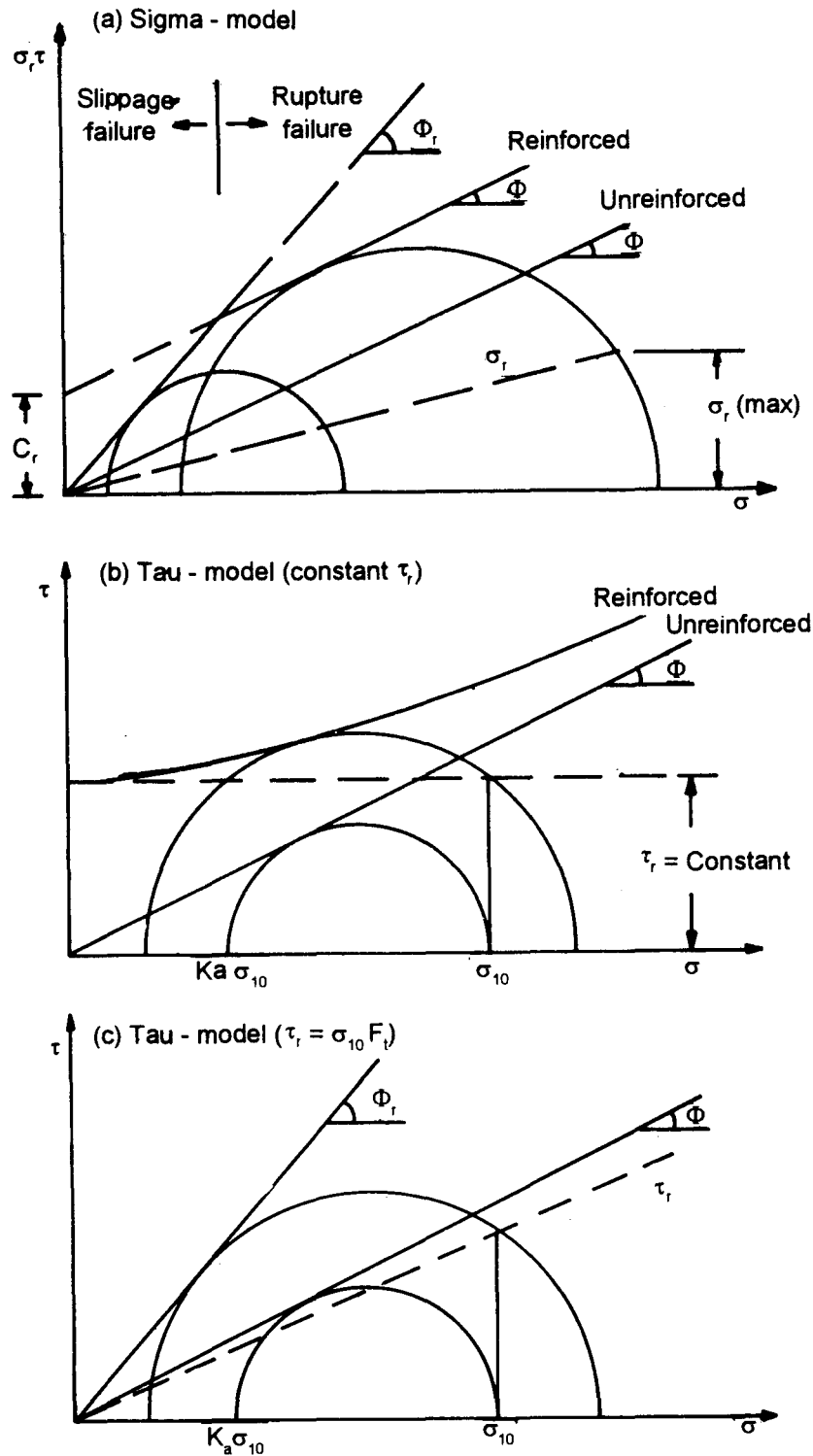
FIGURE 8 Theoretical Strength Models of Reinforced Earth (Hausmann, 1976) (1 m = 3.28 ft)
