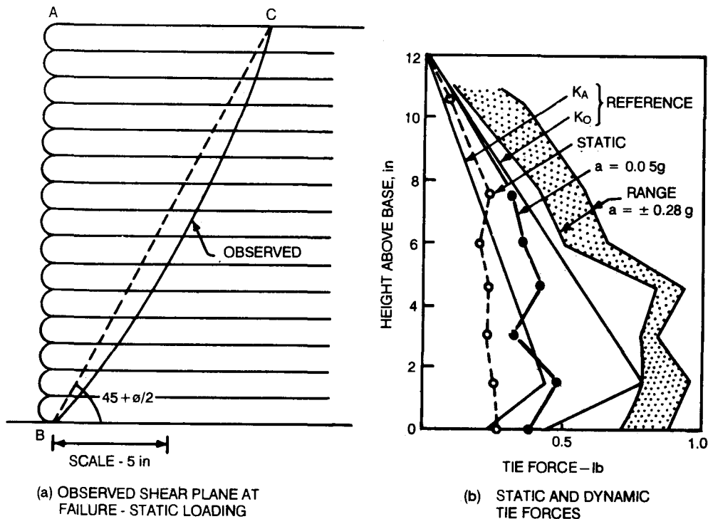
FIGURE 6. Laboratory Model Reinforced Earth Walls
