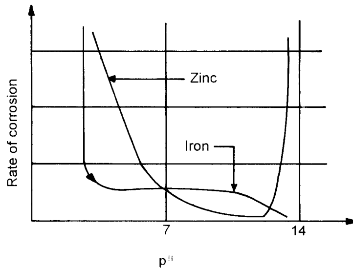
FIGURE 10 Corrosion Rate vs pH
