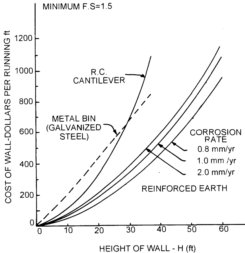
FIGURE 9 Comparative Cost Estimate for Different Types of Walls (1 m = 3.28 ft)
