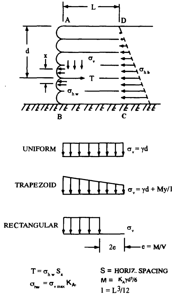
FIGURE 4. Assumption in Some Working Hypotheses on Reinforced Earth Walls
