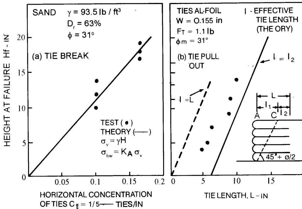
FIGURE 5 TYPICAL MODEL TEST RESULTS TO FAILURE (1 cm = 0.394 inch)
